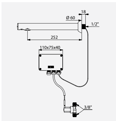
BINOPTIC, lang model DELABIE ref.: 379ENCL
